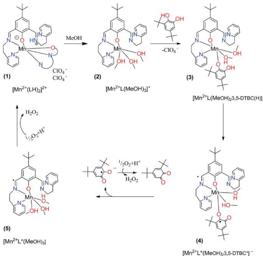
Fig. 6 Proposed mechanistic cycle for catecholase-like activity of complex (1) with 3,5-di-tert-butylcatechol.
