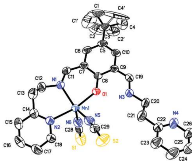
Fig. 3 Molecular structure of compound 3. The disordered domain of the tert -butyl group is indicated by hollow lines. The hydrogen atoms are omitted for clarity. The ellipsoids are drawn at the 50% probability level. Selected bond lengths (Å) and angles (°): Mn1–O1 2.073(2), Mn1–N1 2.185(3), Mn1–N2 2.249(3), Mn1–N5 2.111(3), Mn1–N6 2.091(3), N1–C11 1.271(4), N3–C19 1.280(4), C11–N1–C12 115.7(3), C19–N3–C20 125.6(3).
