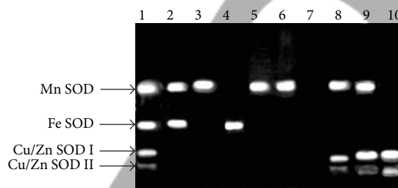
FIGURE 3: Inhibition (KCN, H_2O_2 , and NaN_3 ) study and visualization of SOD isoforms in native PAGE of leaf extracts of Phaseolus vulgaris cv. VL 63 (mother variety) and two SOD-deficient mutant lines, sodPv 1 , and sodPv 2 ; lane 1: mother control (no inhibitor), lane 2: mother variety (KCN), lane 3: sodPv 1 (KCN), lane 4: sodPv 2 (KCN), lane 5: mother variety ( H_2O_2 ), lane 6: sodPv 1 ( H_2O_2 ), lane 7: sodPv 2 ( H_2O_2 ), lane 8: mother variety ( NaN_3 ), lane 9: sodPv 1 , and lane 10: sodPv 2 . Note that complete absence of band at lane 7; Mn SOD is absent in sodPv 2 mutant, and Fe SOD and Cu/Zn SODs are inhibited by H_2O_2 treatment.
