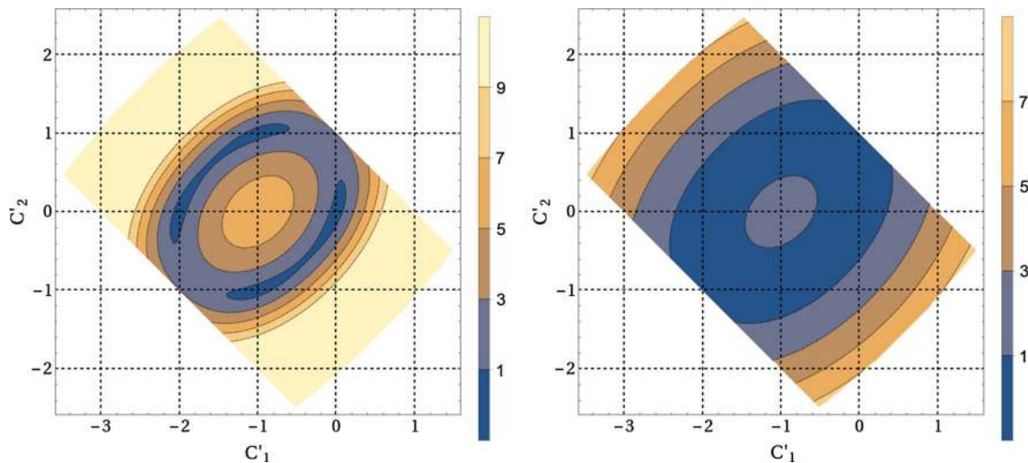
Fig. 4 The contours from the measurement of F'_7 for \mathcal{L}_{\text{int}} = 50 \text{ ab}^{-1} (left), 2 \text{ ab}^{-1} (right)
