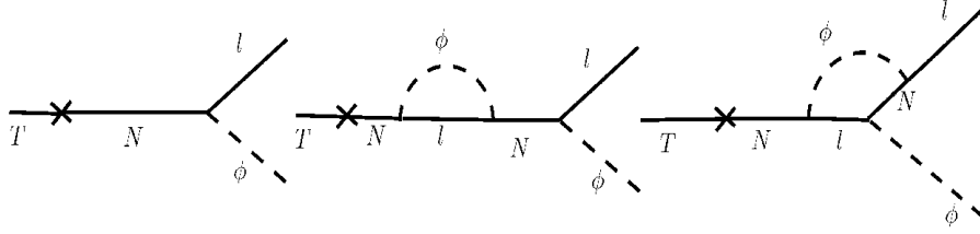
Fig. 1. The tree and one-loop contributions to the decay of T_1 that generate the lepton asymmetry.
