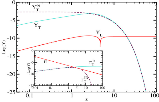
Fig. 2. The comoving density of T_1 - Y_T - and the leptonic asymmetry - Y_L - as a function of z . Also shown is Y_T^{\text{eq}} . The inset displays the decay ( \Gamma_T^D ) and inverse-decay ( \Gamma_T^{\text{ID}} ) rates of T_1 compared with the Hubble expansion rate, H , as a function of z .
