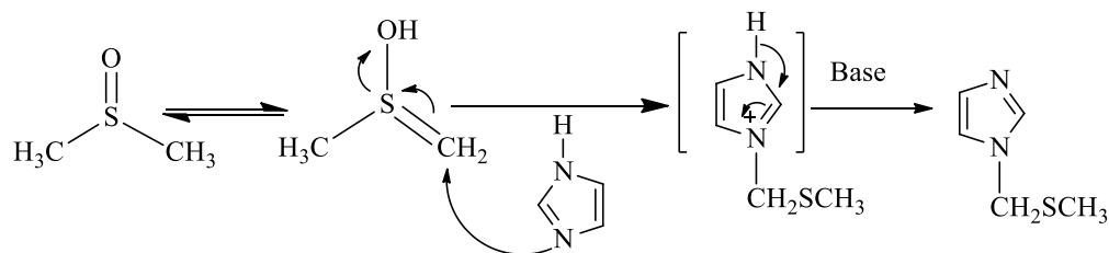
Scheme 2. Probable mechanism for the base catalysed N-methylthiomethylation of imidazole.
