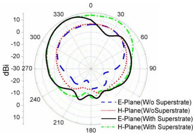
Fig. 4. Simulated radiation patterns of the proposed MIMO antenna 1 with and without (W/o) superstrate in E-plane and H-plane.
