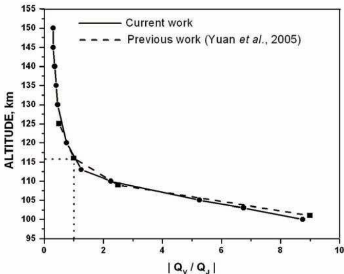
Figure 3. Variation of the ratio of the viscous heating rate to the Joule heating rate with altitude. The continuous curve connecting the filled circles represents the data from the present study, while the dashed curve joining the filled squares represents the data from the earlier study of Yuan et al. [2005].
