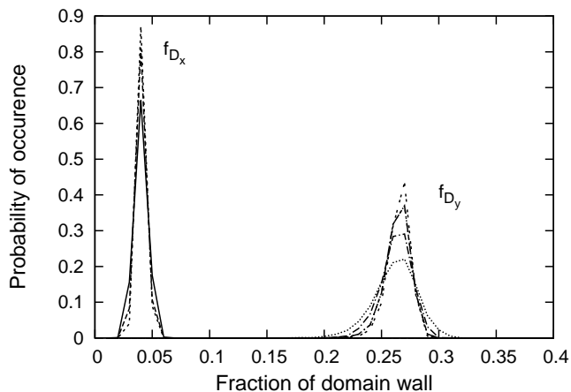
FIG. 9: Steady state distributions of fraction of domain walls at \kappa < 1 for different system sizes. The distributions become narrower as the system size is increased.
