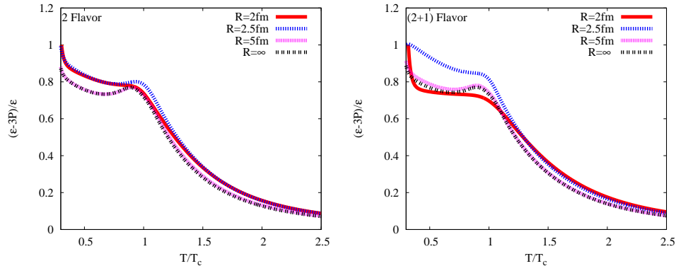
FIG. 6: (Color online) Conformal measure \mathcal{C} = 1 - 3P/\epsilon for different system sizes as a function of temperature.
