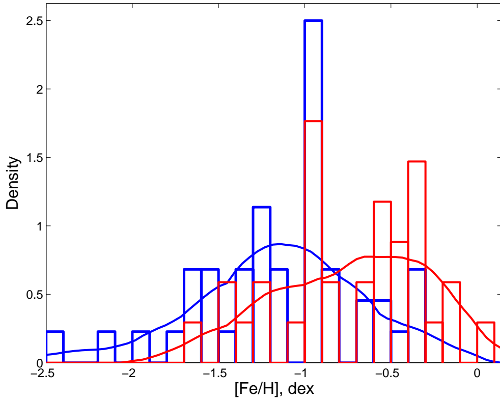
Fig. 4.— Probability density functions of [Fe/H] for the groups G1 and G2. Colors are the same as in Fig2.
