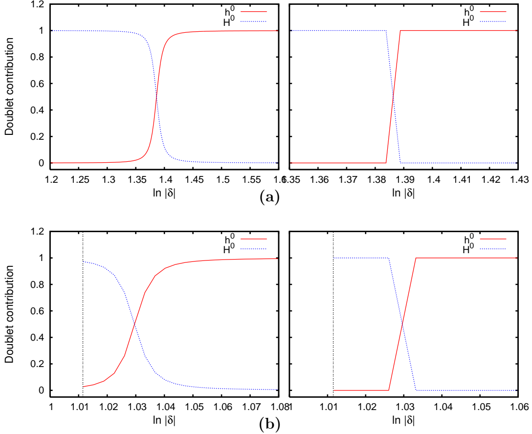
Figure 3: The doublet compositions of h^0 and H^0 as functions of \ln|\delta| . Top left panel: \lambda_i (i = 1 - 5) = 1 and v_2 = 1 GeV. Top right panel: identical with top left but only v_2 = 1 eV. Bottom left panel: identical with top left but only \lambda_1 = 0.7 . Bottom right panel: identical with top left but v_2 = 1 eV, \lambda_1 = 0.7 . For all cases, h^0 remains triplet-dominated below the cross-over point, \ln|\delta| \simeq 1.39 for top panels and \ln|\delta| \simeq 1.03 for bottom panels, beyond which it is doublet-dominated. Just the opposite happens to H^0 . The regions on the left of the vertical line shown in the figures of 2(b) are disallowed, by the chosen lower limits on the scalar masses, such as, M_{H^{++}} > 150 GeV, M_{H^+} , M_{A^0} , M_{H^0} > 100 GeV and M_{h^0} > 115 GeV.
