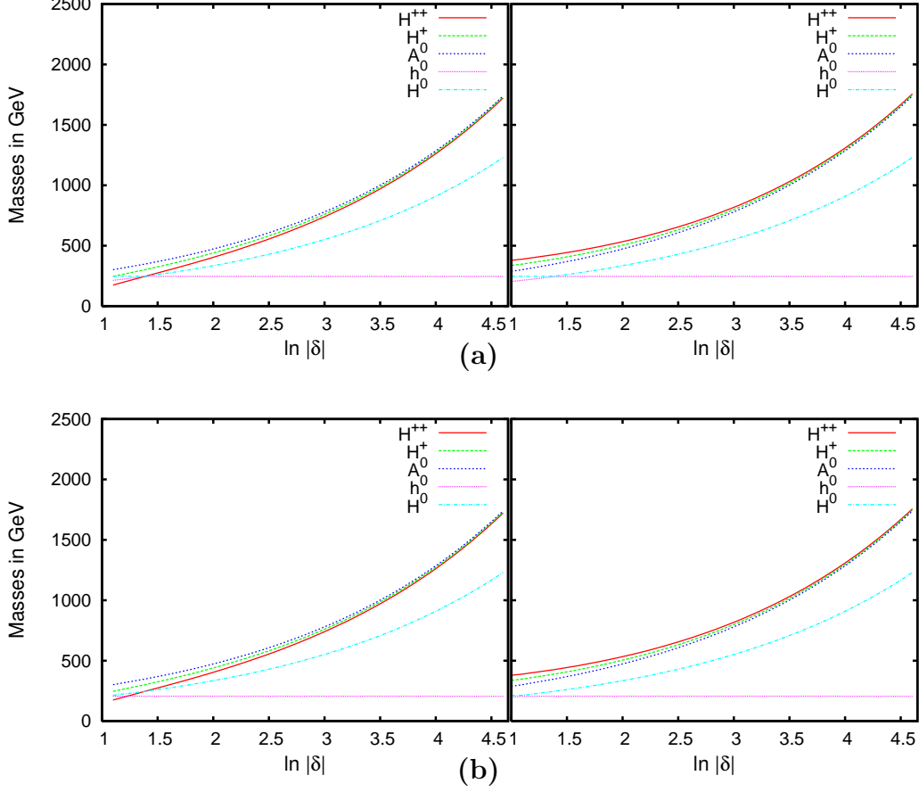
Figure 1: Masses of the scalar physical states as functions of \ln|\delta| ( |\delta| = |a_0/v_2| ). Top left panel: \lambda_i ( i = 1 - 5 ) = 1, v_2 = 1 GeV, and |\delta| varies between 1 and 100, resulting in M_{A^0} > M_{H^+} > M_{H^{++}} . Top right panel: identical with left but only \lambda_4 = -1 , resulting in M_{A^0} < M_{H^+} < M_{H^{++}} . Bottom left panel: \lambda_1 = 0.7 , \lambda_i ( i = 2 - 5 ) = 1, v_2 = 1 GeV, and |\delta| varies between 1 and 100, resulting in M_{A^0} > M_{H^+} > M_{H^{++}} . Bottom right panel: identical with bottom left but only \lambda_4 = -1 , resulting in M_{A^0} < M_{H^+} < M_{H^{++}} . In all these figures the lighter neutral scalar h^0 remains triplet-dominated below the cross-over point, around \ln|\delta| \simeq 1.39 for top left and top right panels and around \ln|\delta| \simeq 1.03 for bottom left and bottom right panels, beyond which it is doublet-dominated. It is just the opposite for H^0 .
