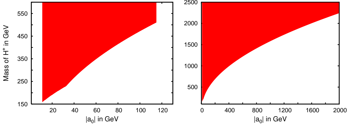
Figure 2: The allowed regions of M_{H^+} - a_0 space, for v_2 < 12 GeV (coming from tree-level upper limit on the \rho -parameter), and M_{h^0} = 120 GeV (left panel) and M_{h^0} = 400 GeV (right panel), are shown by the shaded region marked by red-color. The constraints restricting this parameter space also include those coming from LEP results as well as from the scalar potential (see section 4)
