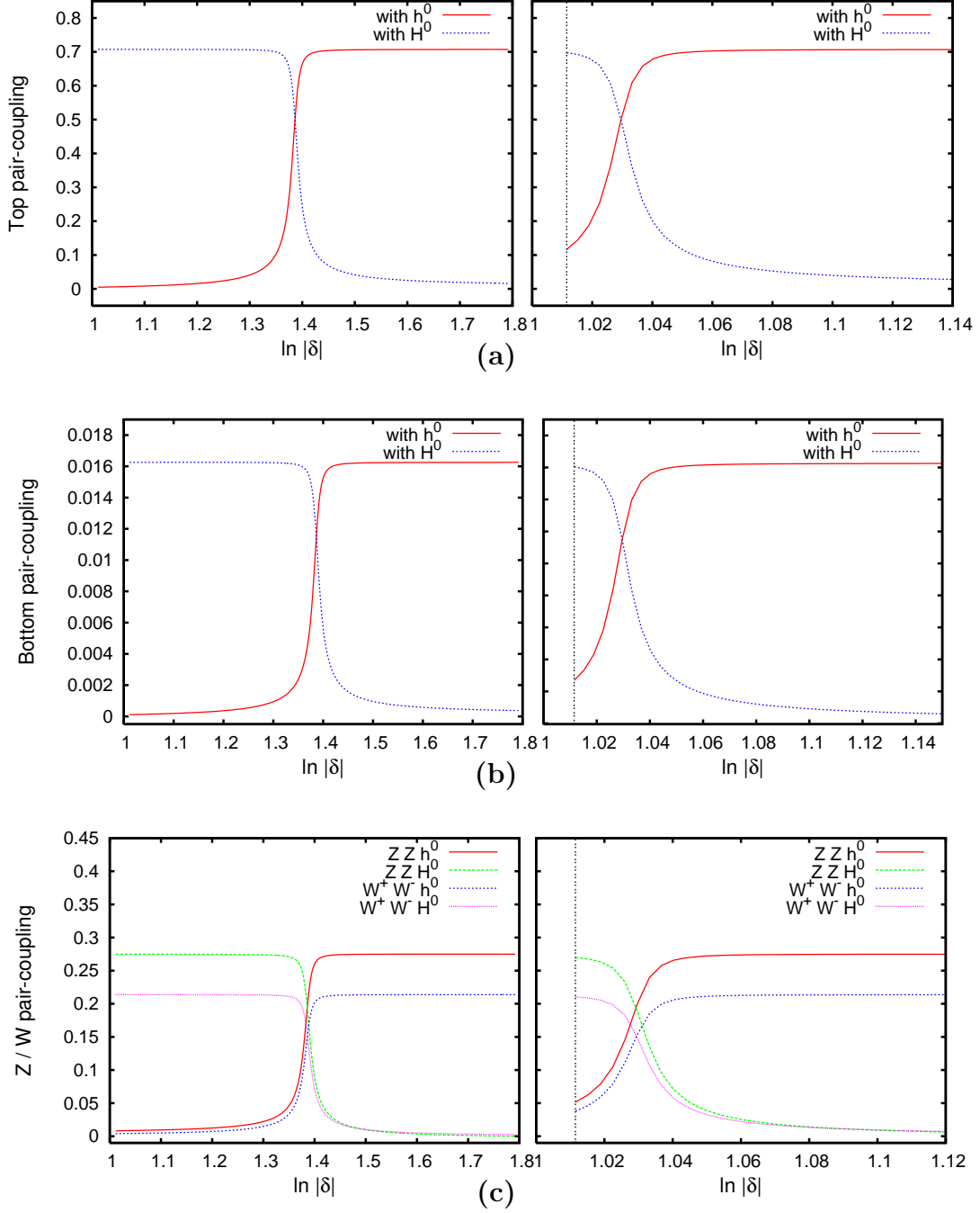
Figure 4: t , b , W^\pm and Z pair couplings with H^0 and h^0 against \ln|\delta| , with \lambda_i ( i = 1 - 5 ) = 1 and v_2 = 1 GeV (in the left panel) and \lambda_1 = 0.7 , \lambda_i ( i = 2 - 5 ) = 1 and v_2 = 1 GeV (in the right panel). Below the cross-over point, \ln|\delta| \simeq 1.39 for left panel and \ln|\delta| \simeq 1.03 for right panel, interactions of h^0 are suppressed, relaxing its experimental mass limit. The regions on the left of the vertical line shown in the figures in the right panel are disallowed, by the chosen lower limits on the scalar masses, such as, M_{H^{++}} > 150 GeV, M_{H^+} , M_{A^0} , M_{H^0} > 100 GeV and M_{h^0} > 115 GeV.
