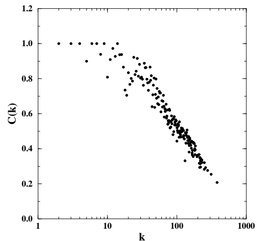
FIG. 3: The variation of the clustering coefficient C(k) against the degree k for the IRN indicates a logarithmic decay for large k .
