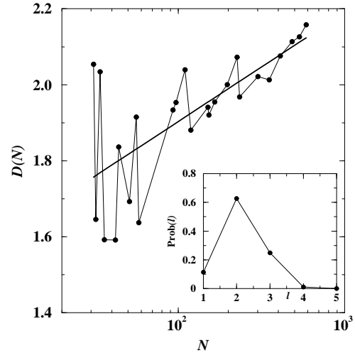
FIG. 1: The variation of the mean distance D(N) of 25 different subsets of IRN having different number of nodes ( N ). The whole range is fitted with a function like D(N) = A + B \log(N) where A \approx 1.33 and B \approx 0.13 . The inset shows the distribution \text{Prob}(\ell) of the shortest path lengths \ell on IRN. The lengths varied to a maximum of only five link lengths and the network has a mean distance D(N) \approx 2.16 .
