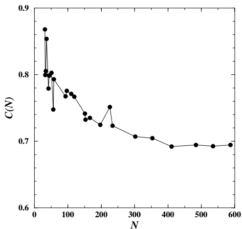
FIG. 2: Variation of the clustering coefficient C(N) of 25 different subsets of IRN having different number of nodes N . Starting from a somewhat higher value at small number of nodes, the clustering coefficient decreases slowly on increasing N and finally saturates at 0.69.
