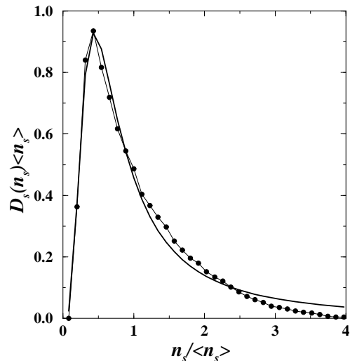
FIG. 6: Scaled probability distribution D_s(n_s) for an arbitrary train passing through n_s stations where \langle n_s \rangle \approx 12.37 . Binned data is presented through the black dots connected by lines which fits best to the form: D_s(n_s)\langle n_s \rangle = ax^4/(x^2 + b)^3 with x = n_s/\langle n_s \rangle , a \approx 0.6 and b \approx 0.096 .
