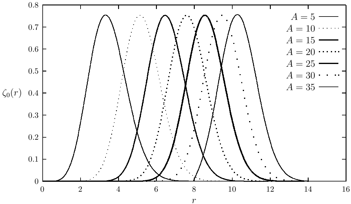
Fig. 6 - Plot of ground state wave function as a function of hyperradius ( r ) for various indicated value of A , in the chosen trap.
