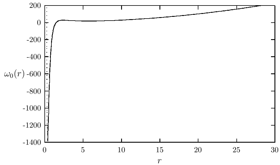
Fig. 4 - Plot of \omega_0(r) as a function of r (dotted and continuous curves together) for A = 16 (critical number) for the same attractive two-body potential as in Fig. 3.
