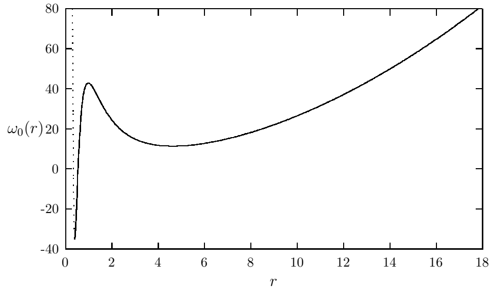
Fig. 3 - Plot of \omega_0(r) as a function of r (dotted and continuous curves together) for A = 10 (subcritical number) for a model attractive two-body interaction ( V_0 = -100 o.u., r_0 = 0.0855 o.u.), which corresponds to a_{sc} = -0.1176 o.u.
