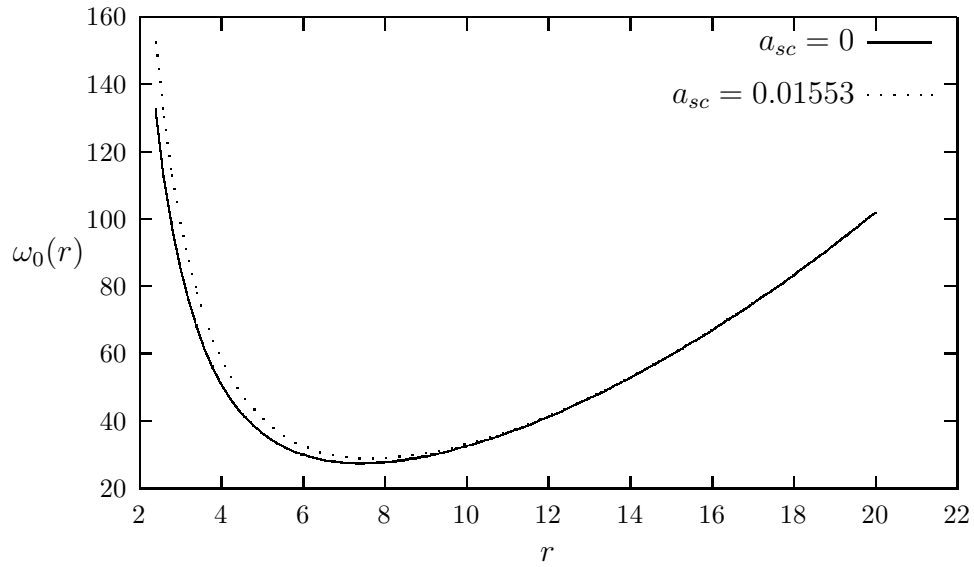
Fig. 2 - Lowest eigen potential for A = 20 as a function of r . Continuous curve is for a_{sc} = 0 (no two-body interaction) and the dotted curve is for a repulsive interaction ( a_{sc} = 0.01553 o.u.).
