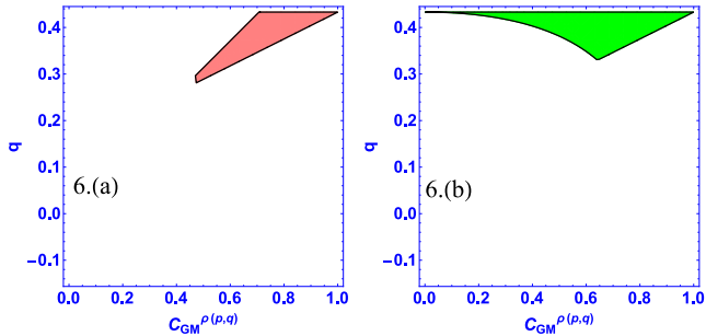
FIG. 6: Variation of state parameter q with that of C_{GM}^{\rho(p,q)} for genuinely nonlocal states are shown in these figures. The genuinely nonlocal states, as detected by Svetlichny inequality and 99-th facet inequality are considered separately in Fig.(a) and Fig.(b) respectively. It is interesting to note that for any positive value of C_{GM}^{\rho(p,q)} , there exist some states whose genuine nonlocality is observed via violation of 99-th facet. However for the states whose genuine nonlocality is guaranteed by the violation of Svetlichny inequality, no such conclusion can be made. In fact for violation of Svetlichny inequality, the range of C_{GM}^{\rho(p,q)} gets restricted : C_{GM}^{\rho(p,q)} > \sqrt{2} - 1
