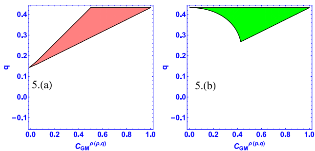
FIG. 5: Both of these figures depict variation of C_{GM}^{\rho(p,q)} with state parameter q for standard nonlocal states. Precisely, in Fig.(a) and Fig.(b), we have considered C_{GM}^{\rho(p,q)} of the states whose standard nonlocality is guaranteed by violation of Mermin and 15-th facet inequality respectively. Interestingly, for any arbitrarily small value of C_{GM}^{\rho(p,q)} there exists at least one GHZ-symmetric state which exhibits standard nonlocality.
