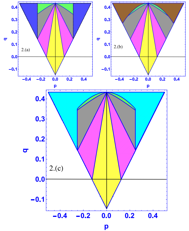
FIG. 2: (a) The blue areas represent the nonlocal region obtained via the violation of Mermin inequality (Eq.5). (b) Regions of violation of 15-th inequality are given by the brown regions. Clearly, the regions restricted by p \leq \frac{1}{4} in the brown regions indicate the areas where 15-th facet inequality (Eq.(11)) emerges as a more efficient tool over Mermin inequality (Eq.5) for revealing nonlocal nature of GHZ-symmetric states. (c) The cyan areas give the optimal region of standard nonlocality of GHZ-symmetric states. The states characterized by the state parameters lying in this region, when shared between Alice, Bob and Charlie do not admit any local hidden variable model.
