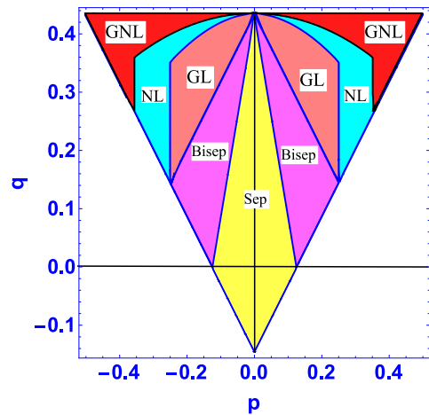
FIG. 4: The figure gives the nonlocality classification of three qubit GHZ-symmetric states \rho(p, q) . The red regions give the optimal area where genuine nonlocality (GNL) is revealed with respect to projective measurement for GHZ-symmetric states. The cyan regions indicate the optimal area where standard nonlocality (NL) is revealed (except genuine nonlocality). As genuine nonlocality also implies standard nonlocality so red regions also give the region of standard nonlocality. Genuinely entangled but local states (GL) are represented by pink regions. Clearly, no nonlocal region lies within biseparable region (Magenta).
