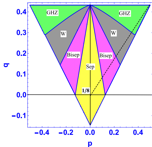
FIG. 1: The triangle of the GHZ-symmetric states for three qubits [36]. The upper corners of the triangle are the standard GHZ states |GHZ_+\rangle and |GHZ_-\rangle . Mixed state \frac{1}{8} is located at the origin. The black dashed line represents the generalized Werner state. We have indicated different types of three qubit entanglement: GHZ (green), W (grey), Biseparable (magenta), Separable (yellow).
