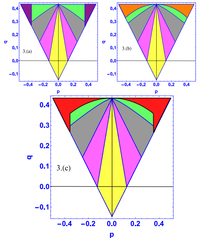
FIG. 3: (a) The purple areas give the restricted region of state parameters for which genuine nonlocality of the corresponding states is guaranteed by violation of Svetlichny inequality(Eq.7). (b) Analogously, the orange regions represent the areas where genuine nonlocality is observed due to violation of 99-th facet inequality(Eq.(15)). Now the regions restricted by |p| \leq \frac{1}{2\sqrt{2}} in the orange regions give the the areas where the 99-th facet serves as a better tool to exploit genuine nonlocality of GHZ-symmetric states compared to Svetlichny inequality. (c) The optimal region of nonlocality of GHZ-symmetric states is given by the red regions.
