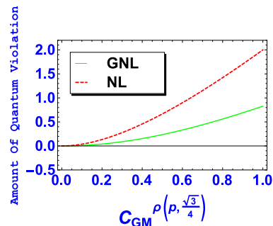
FIG. 7: The red dashed curve gives variation of amount of standard nonlocality( L_{max} - 4 ) with the amount of entanglement( C_{GM}^{\rho(p,q)} ) whereas the solid green curve represents the variation of amount of genuine nonlocality( NS_{max} - 3 ) with the amount of entanglement( C_{GM}^{\rho(p,q)} ). The figure shows that standard nonlocality(NL) and genuine nonlocality(GNL) both are obtained for any positive value of C_{GM}^{\rho(p,q)} . The curve showing variation of GNL with C_{GM}^{\rho(p,q)} for this mixed subclass of GHZ-symmetric states is same as that of the curve showing variation of GNL with C_{GM}^{\rho(p,q)} for pure generalized GHZ State[33].
