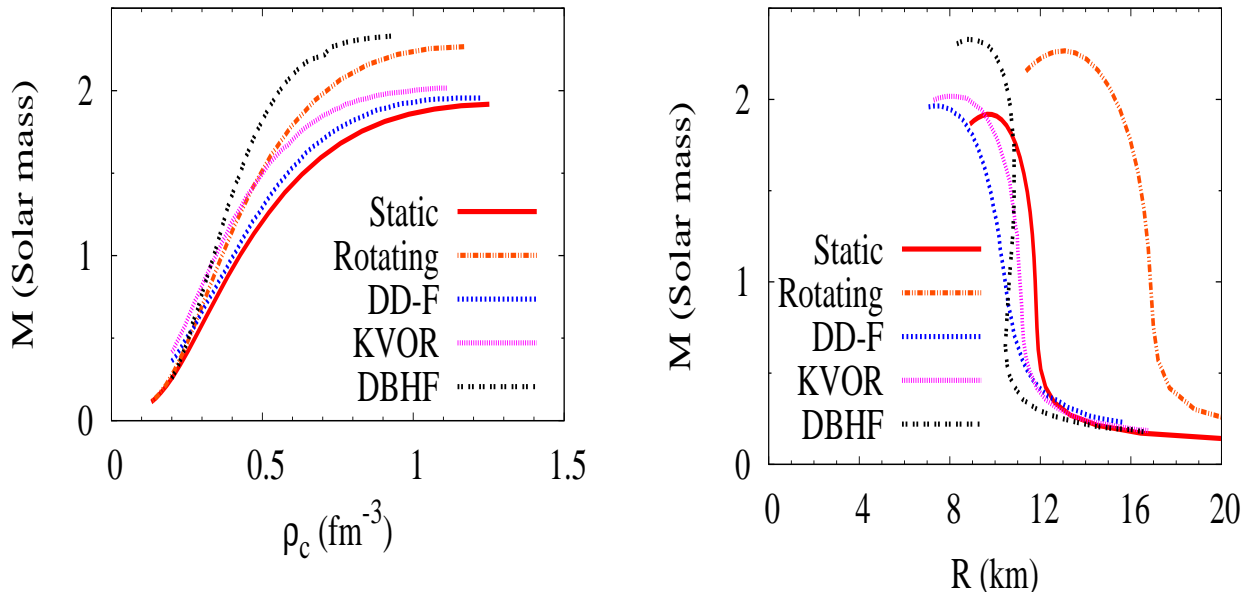
FIG. 2. (Color online) (a) (Left) The variation of NS masses ( M ) is shown with central density ( \rho_c ). The results of this calculation are denoted as ‘Static’ and ‘Rotating’ for non-rotating and rotating NSs at the Keplerian limit. (b) (Right) Mass-Radius relationship is given for static and rotating stars at Keplerian frequency using this EoS. The other three plots (DD-F, KVOR, DBHF) present the same relationship for static star only.
