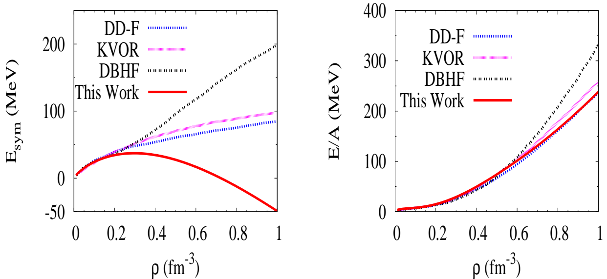
FIG. 1. (Color online) (a) (Left) Density dependent behavior of symmetry energy ( E_{sym} vs. \rho ) determined by different approaches. (b) (Right) The EoS determined by different models ( E/A vs. \rho ) are shown for beta equilibrated charge neutral neutron star matter.
