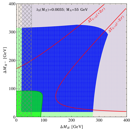
FIG. 2. The allowed parameter space in \Delta M_H - \Delta M_{H^\pm} plane for M_A = 55 GeV and \lambda_S = 0.0035 . The constraints from the T parameter, LEP II and the stronger unitarity condition are as in Fig. 1. The blue region is allowed by the DM constraint at the 3\sigma level [5] and the weaker unitarity condition.
