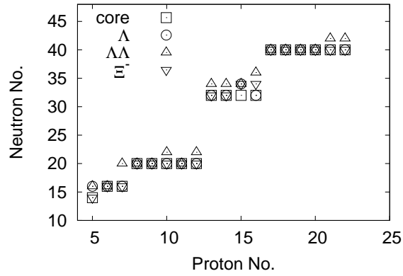
Figure 2: Neutron driplines of single- \Lambda , double- \Lambda , \Xi^- hypernuclei as compared to that of the normal nuclei for Z \leq 22 .
