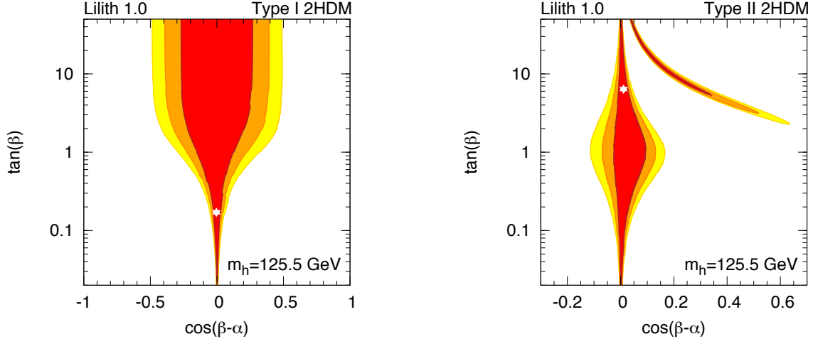
Figure 1: The red, orange and yellow regions represent the 68%, 95% and 99% C.L. allowed regions, respectively, coming from the Higgs signal strength measurements at the LHC. The left (right) panel shows the situation for Type I (II) model. The star-marked points correspond to the best fit values (figures adapted from [23]).
