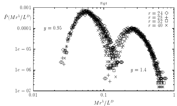
FIG. 4. The partial collapses of the data for the scaled distribution \tilde{P}(Mr^y/L^D) = P(M/L^D)r^{-y\zeta} for ranks r = 24, 28, 32 and 40 with two different values of y are shown separately.
