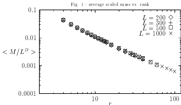
FIG. 1. Variation of the average \langle M/L^D \rangle against the ranks are shown for lattice sizes L = 200, 300, 500 and 1000 . Larger number of data (corresponding to higher ranks) are available for increasing lattice size.
