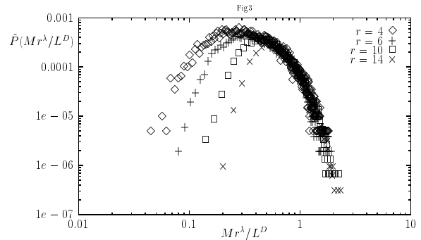
FIG. 3. The partial collapse of the data for the scaled distribution \tilde{P}(Mr^\lambda/L^D) = P(M/L^D, r)r^{-y\zeta} is shown for ranks r = 4, 6, 10 and 14 . The value of y is 1.75 here.
