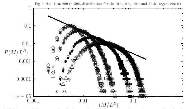
FIG. 2. The probability distribution for the ranked cluster masses are shown for ranks r = 4, 6, 10 and 14 (from right to left) for lattice sizes L = 200, 300, 400 and 500 against the scaled masses. The peaks of the distribution show a power law behaviour with M/L^D where the maxima occur for each rank.
