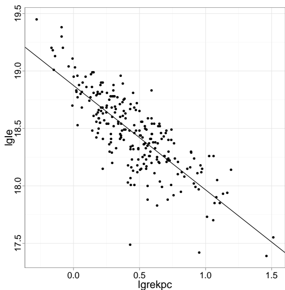
Figure 6: A plot showing the best-fit line between effective radius of the galaxy and its average surface brightness i.e. the Kormendy plot.
