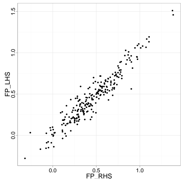
Figure 4: A plot between the left-hand-side vs the right-hand-side of the Equation 2, often referred to as the edge-on view of the plane.
