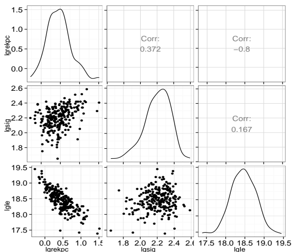
Figure 5: A pairs plot generated by AstroStat. The plot on the bottom-left corner is the Kormendy plot which relates effective radius of the galaxy with its average surface brightness.
