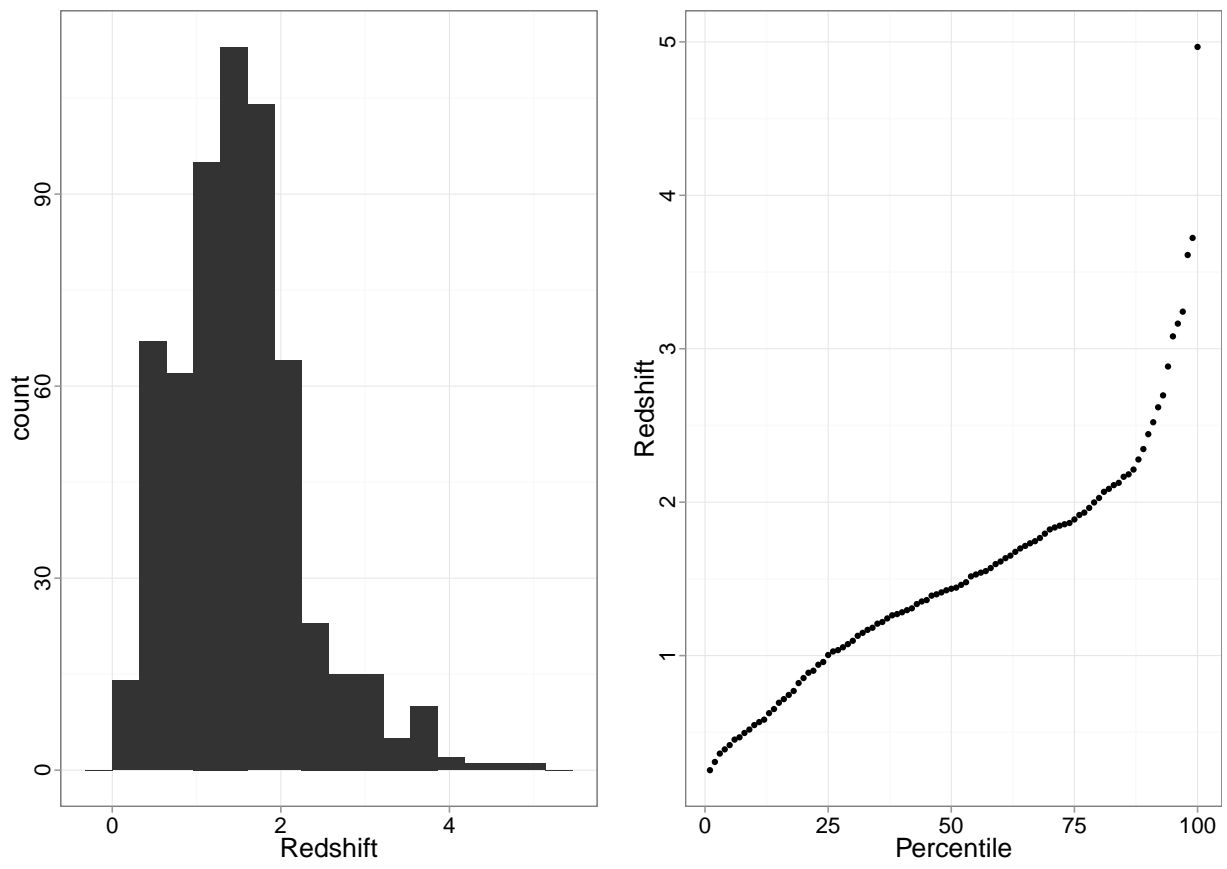
Figure 9: A histogram and a quantile plot generated using ggplot2.
