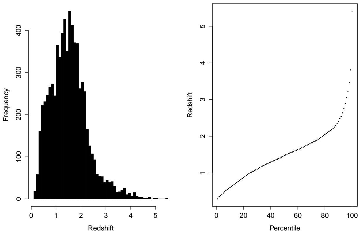
Figure 8: A histogram and a quantile plot generated using base graphics in R.
