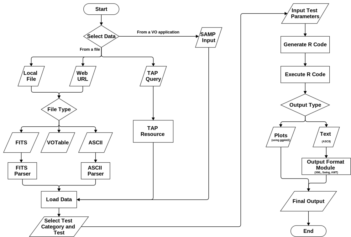
Figure 3: A flowchart showing the inner workings of AstroStat.
