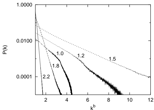
FIG. 6: The degree distribution is plotted against k^b to show the stretched exponential behaviour for several values of \lambda (the labels denote the values of \lambda ). The values of b are 0.1, 0.20, 0.42, 0.3 and 0.2 for \lambda = 2.2, 1.8, 1.5, 1.2, 1.0 respectively.
