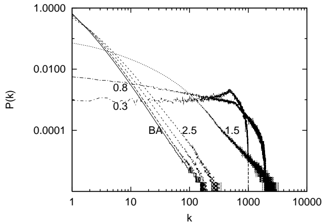
FIG. 5: The degree distribution for the stochastic model for several values of \lambda (denoted by the labels) are shown. In between the BA curve and the curve for \lambda = 2.5 , the two unlabelled curves correspond to \lambda = 4.0 and \lambda = 3.0 . For higher values of \lambda , the network is grown to 4000 nodes while for the lower-most \lambda , we have maximum 1000 nodes.
