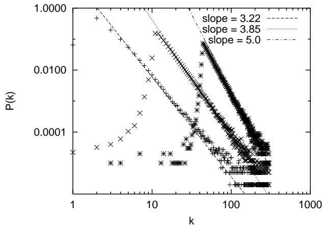
FIG. 2: The normalised degree distribution in the deterministic network for \theta = 0.1, 0.3 and 0.5 are shown along-with straight lines in the log-log plot which have slopes according to equation (6). For \theta = 0.1 and 0.3 , t = 4000 and for \theta = 0.5 , t = 2000 .
