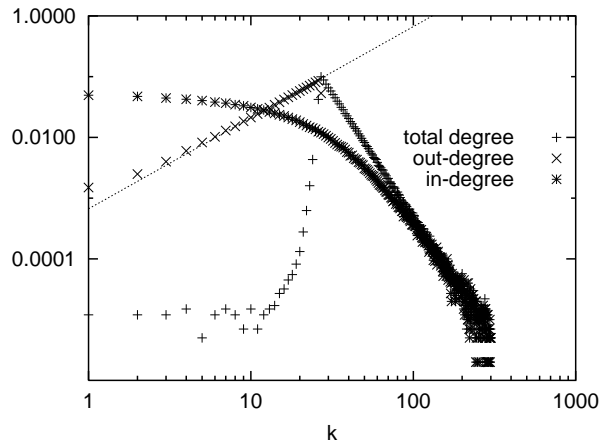
FIG. 3: The in-degree, out-degree and total degree distributions for \theta = 0.4 are shown. P_{out}(k_{out}) is fitted with the calculated slope given by eq. 8.
