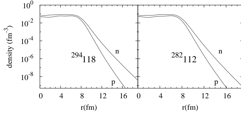
FIG. 1: Calculated nucleon densities in ^{294}_{118} and ^{282}_{112} . Here n(p) refer to neutron(proton) densities, respectively.
